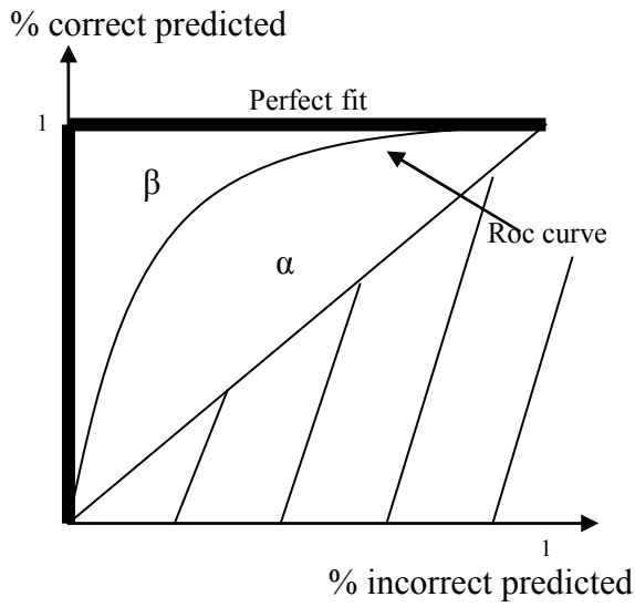
Figure 4. Illustrating the ROC-curve idea
