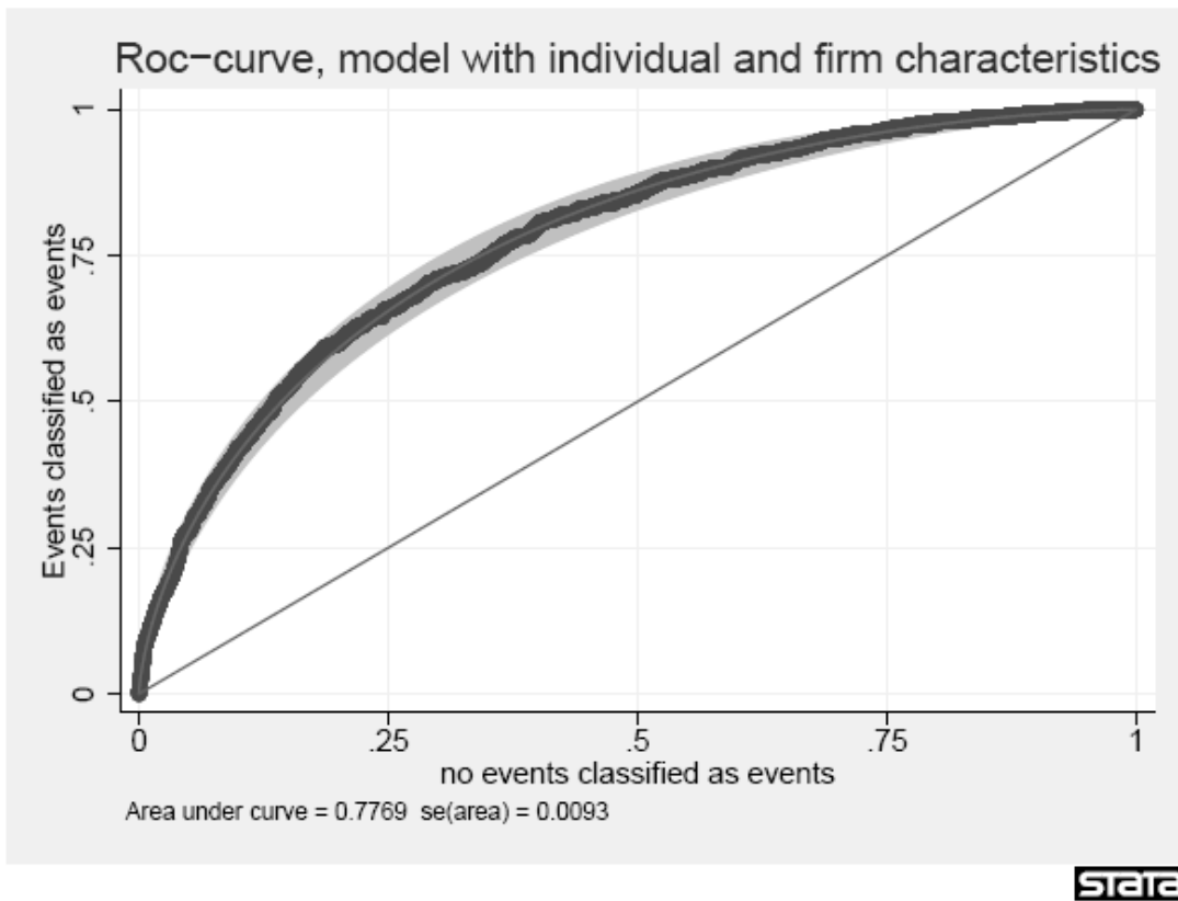
Figure 5. The ROC curve for the extended model
