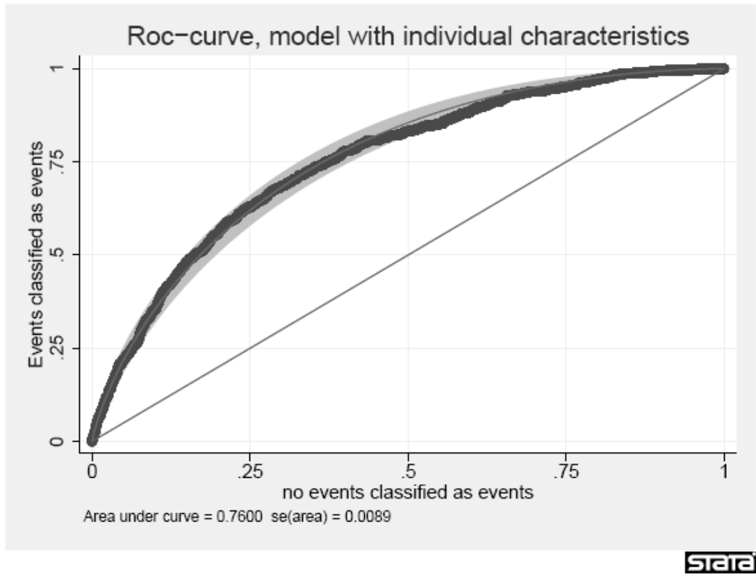
Figure 6. The ROC curve for the basic model
