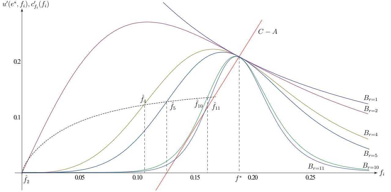
Figure 2: Single crossing in equation (37) ensures a unique global maximum at f_i = f^* for the example setup of section 3.1. The dotted line gives the location of inflection points \hat{f} for different r .
