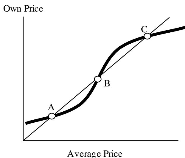
Figure 3: Best reply structure with multiple equilibria
